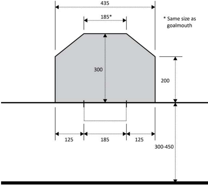
Diagram 2. Alternate Version Crease
